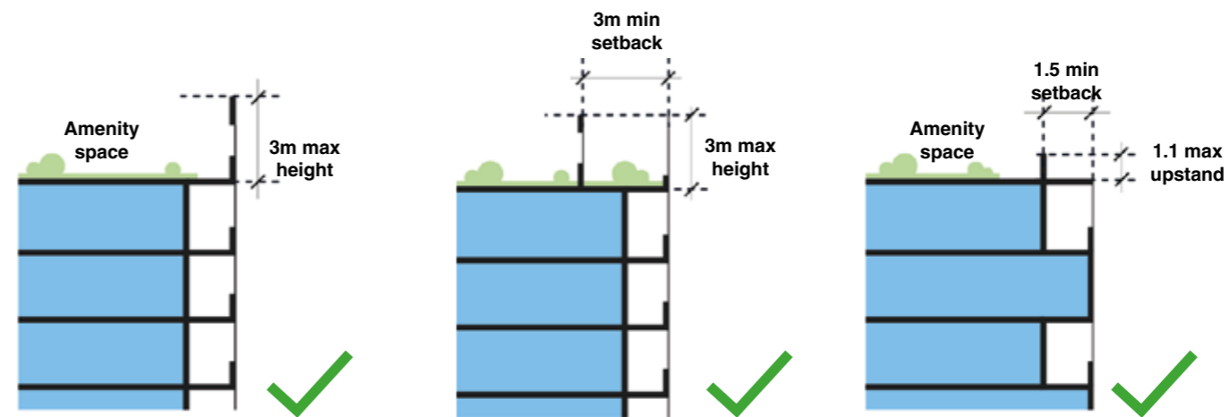
Figure 5.130 Façade overrun
