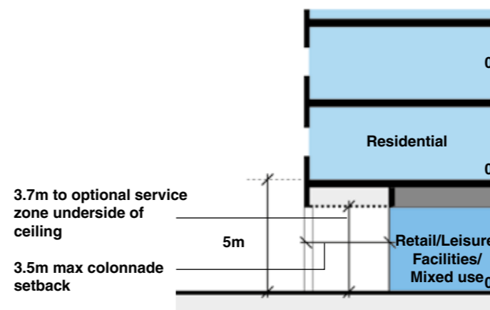
Figure 5.70 Colonnade section
