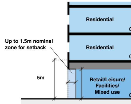
Figure 5.69 Frontage Setback at 1.5m
