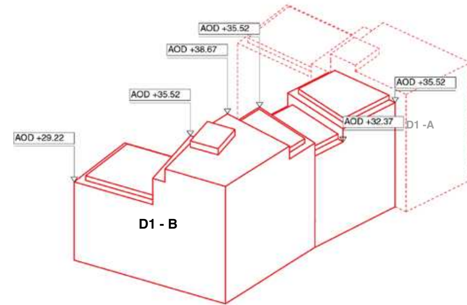
Figure 6.341 Plot D1B Maximum plot parameters showing shoulder heights
