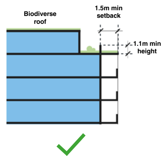
Figure 6.268 Upstand to 1.1m min height and a 1.5m min setback
