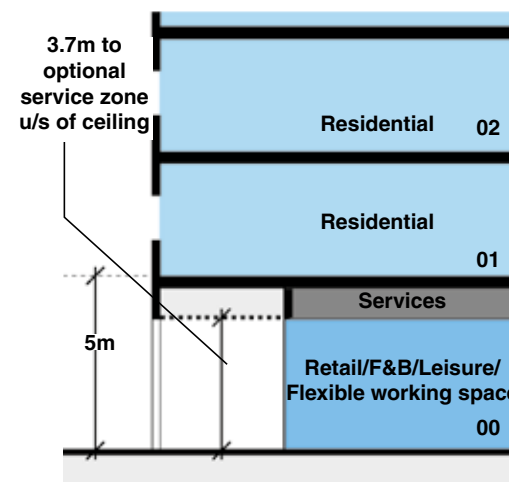
Figure 6.198 Colonnade at ground floor condition
