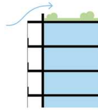
Figure 6.76 1.1m balustrade upstands for wind mitigation
