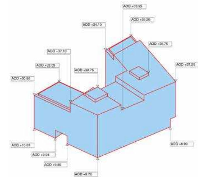
Figure 6.4 Maximum plot parameters diagram - View 02
