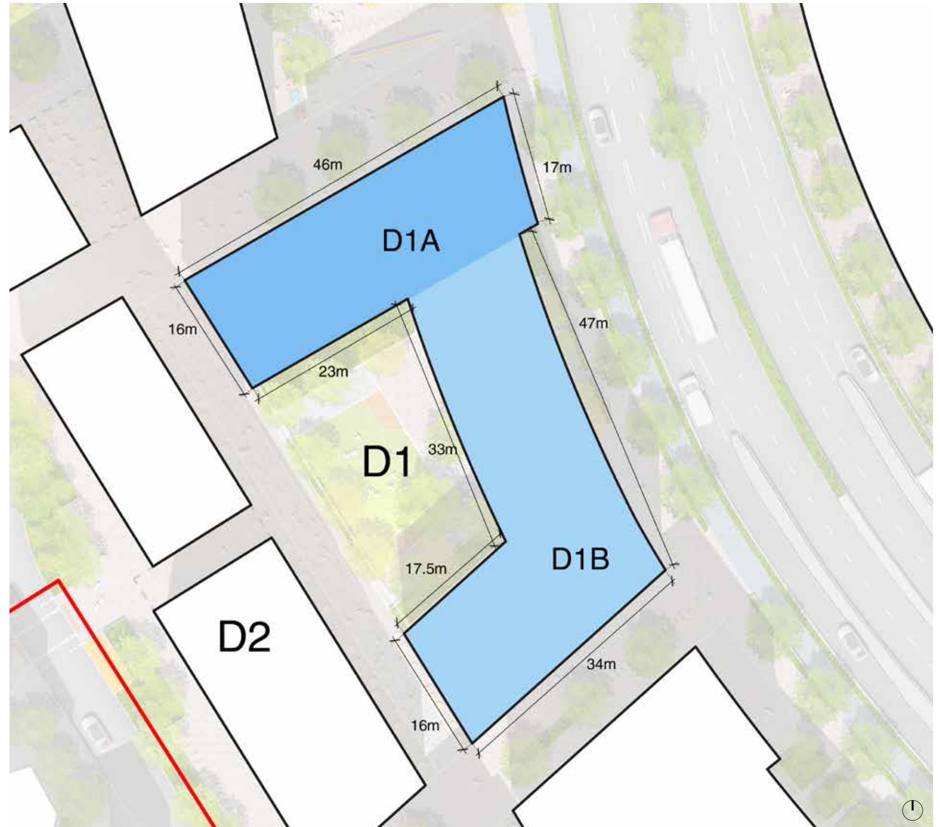
Figure 6.324 Ground floor plan
