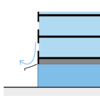
Figure 6.75 Awning wind mitigation
