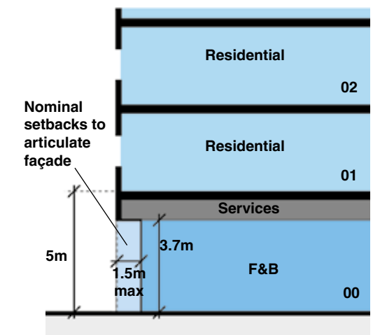
Figure 6.279 Up to 1.5m nominal setback condition
