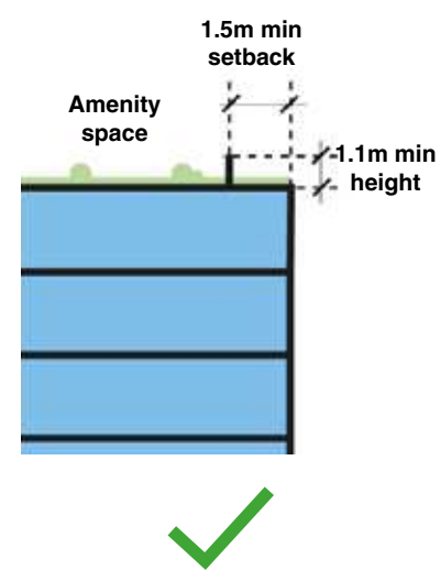
Figure 6.267 Upstand to 1.1m min height and a 1.5m min setback
