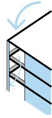
Figure 6.332 Inset balconies on corners for wind mitigation
