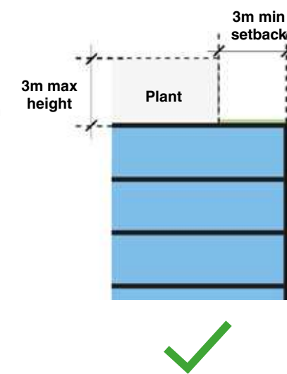
Figure 6.269 Single storey with plant setback
