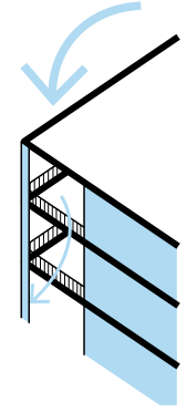
Figure 6.166 Inset balconies on corners for wind mitigation
