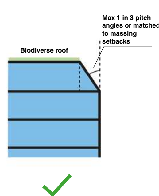
Figure 6.186 Single storey mansard or pitched roof
