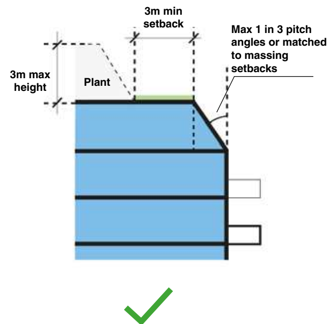
Figure 6.185 Single storey mansard or pitched roof with plant setback
