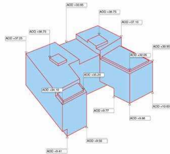
Figure 6.3 Maximum plot parameters diagram - View 01
